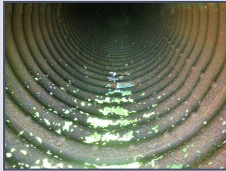
Severely corroded principal spillway pipe in Jefferson County.
