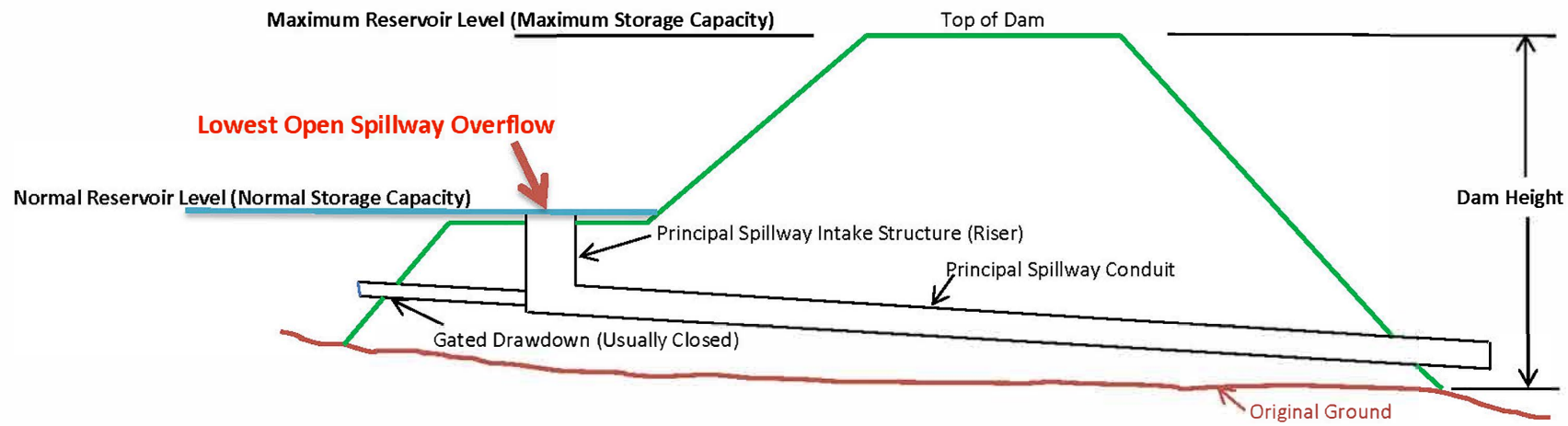
CROSS-SECTION VIEW
