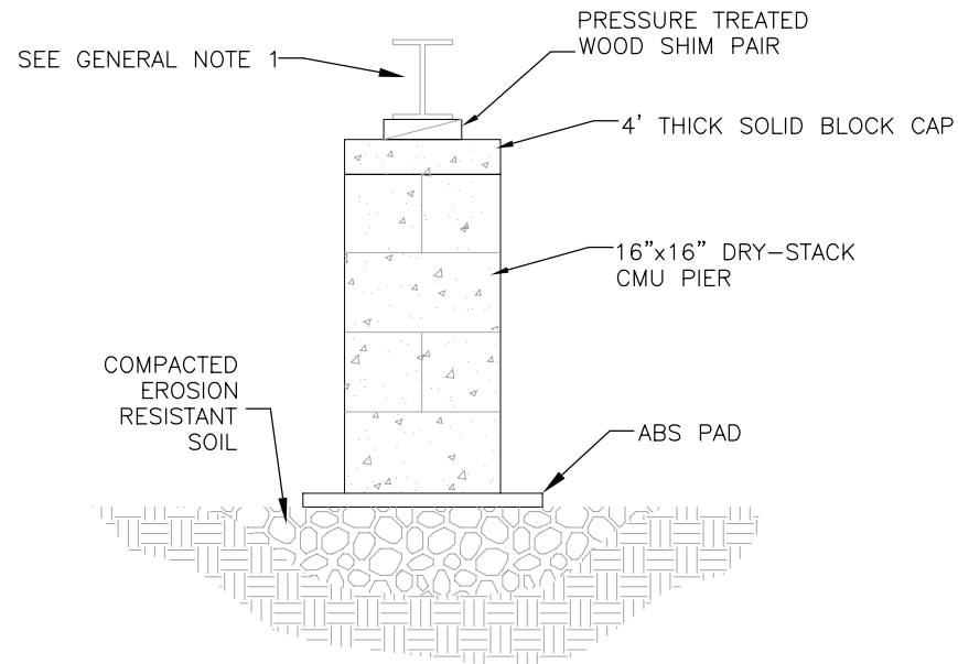
ALTERNATIVE MASONRY PIER DETAIL FOR FLOOD VELOCITIES UP TO 1.25 FT/SEC
