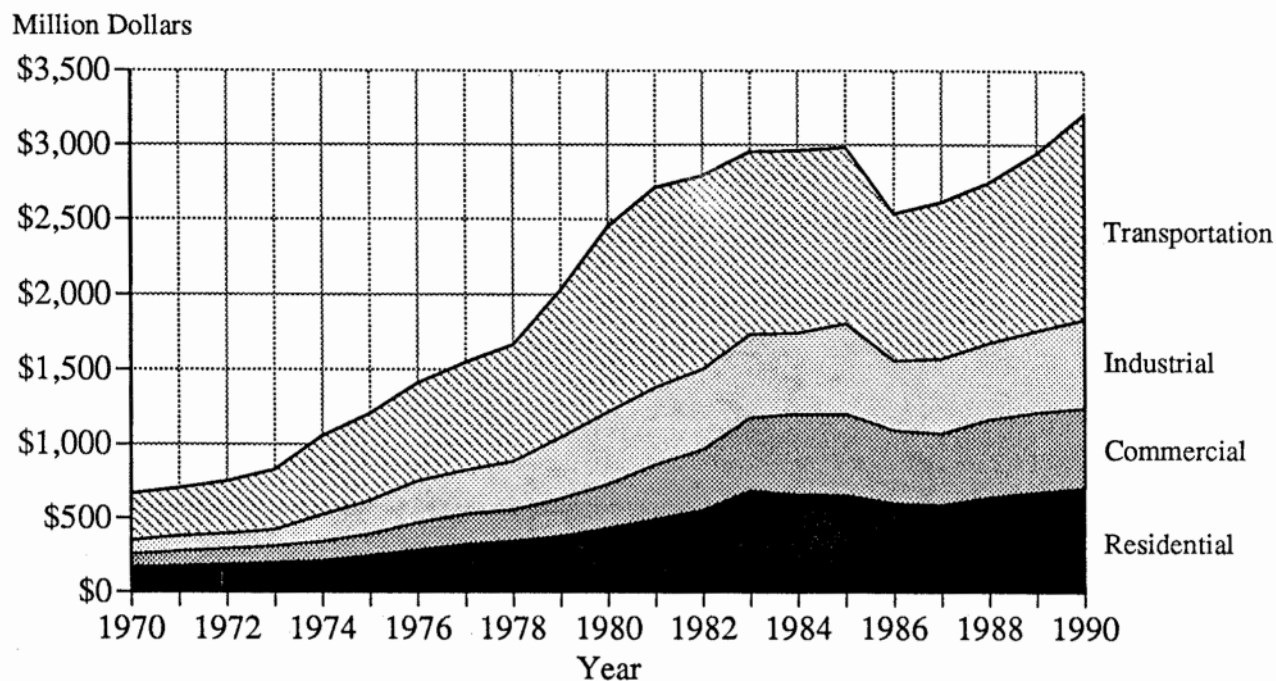
Figure 7 Expenditures by End-Use Sector, Nebraska, 1970-1990
