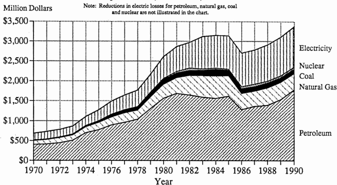
Figure 6 Total Expenditures, Nebraska, 1970-1990
