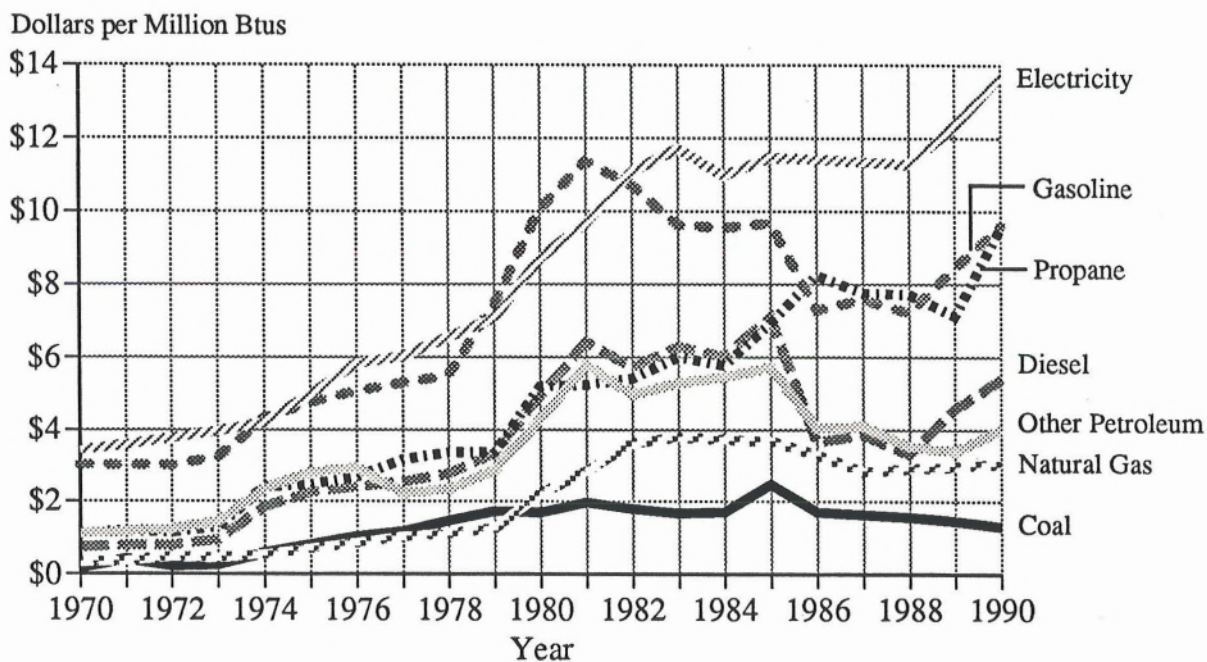
Figure 21 Prices by Fuel Type, Nebraska, 1970-1990
