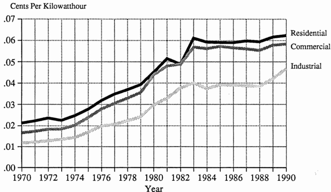
Figure 58 Prices by Sector, Nebraska, 1970-1990
