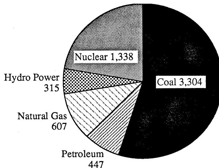
Generator Nameplate* by Energy Source, Nebraska, 1990 (Megawatts)
