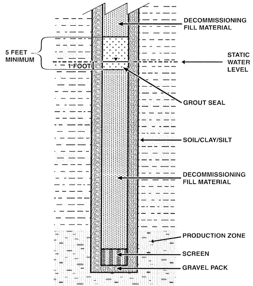
FIGURE 16. DECOMMISSIONING DRILLED WELLS
