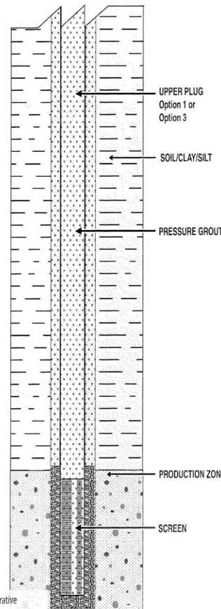
FIGURE 19. DECOMMISSIONING FULL LENGTH GROUTED WELLS
