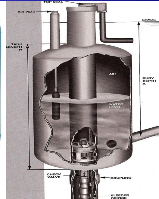
Steel Buried Hydro-Pneumatic Tank with Air Volume Control System
