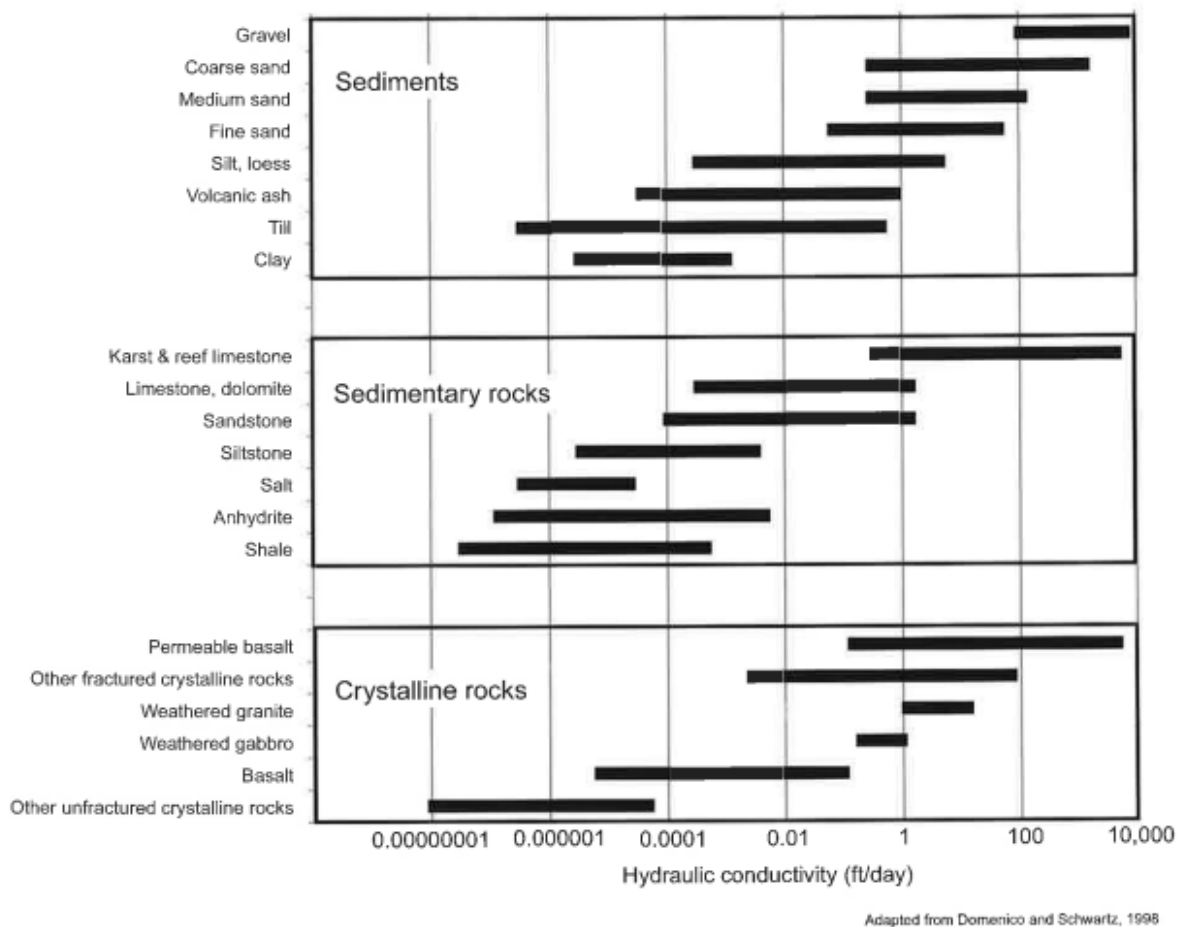
Figure 9. Ranges of hydraulic conductivity (permeability relative to water) for different sediments and rocks. Due to extremely large range of values, horizontal scale is logarithmic so that each division from left to right marks a hundred fold increase from the previous division.
