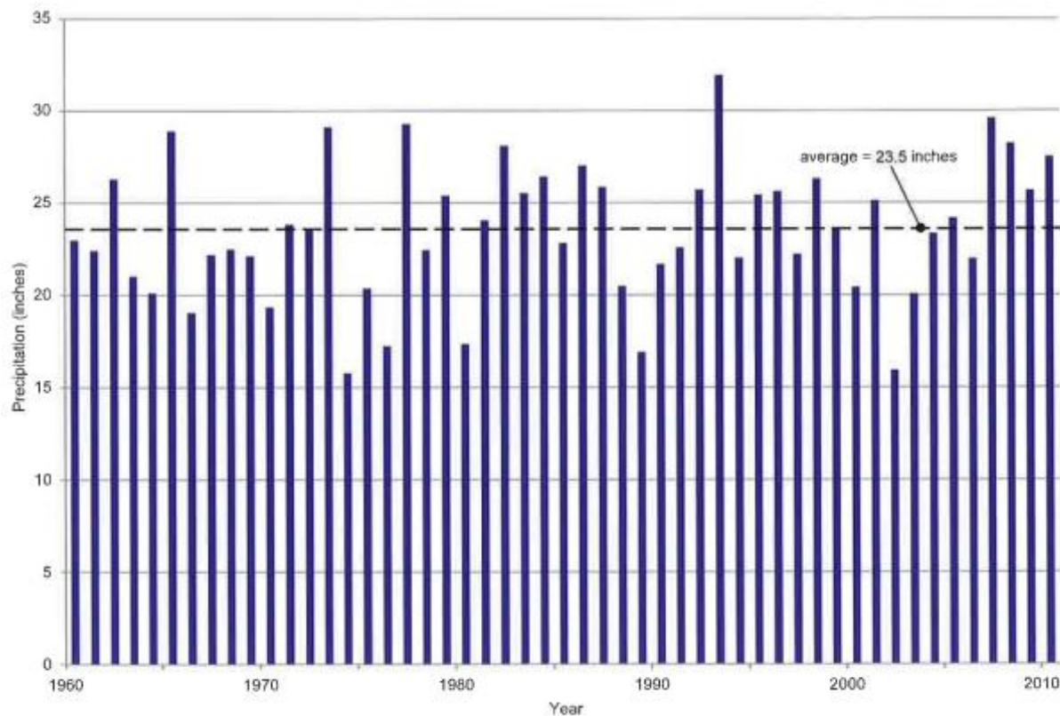
Figure 25. Average annual statewide precipitation from 1960 to 2010.
