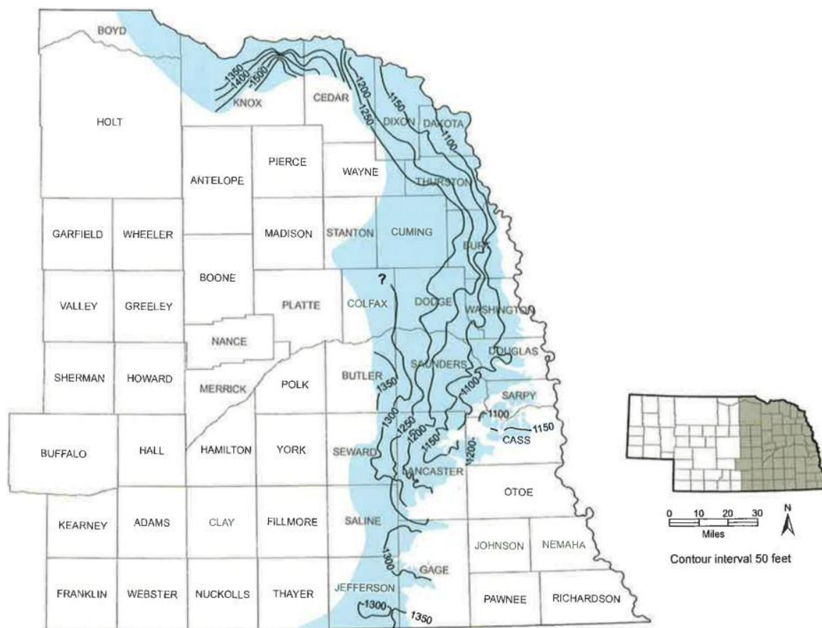
Figure 30. Elevation of the water table or potentiometric surface of the Maha (Dakota) aquifer.
