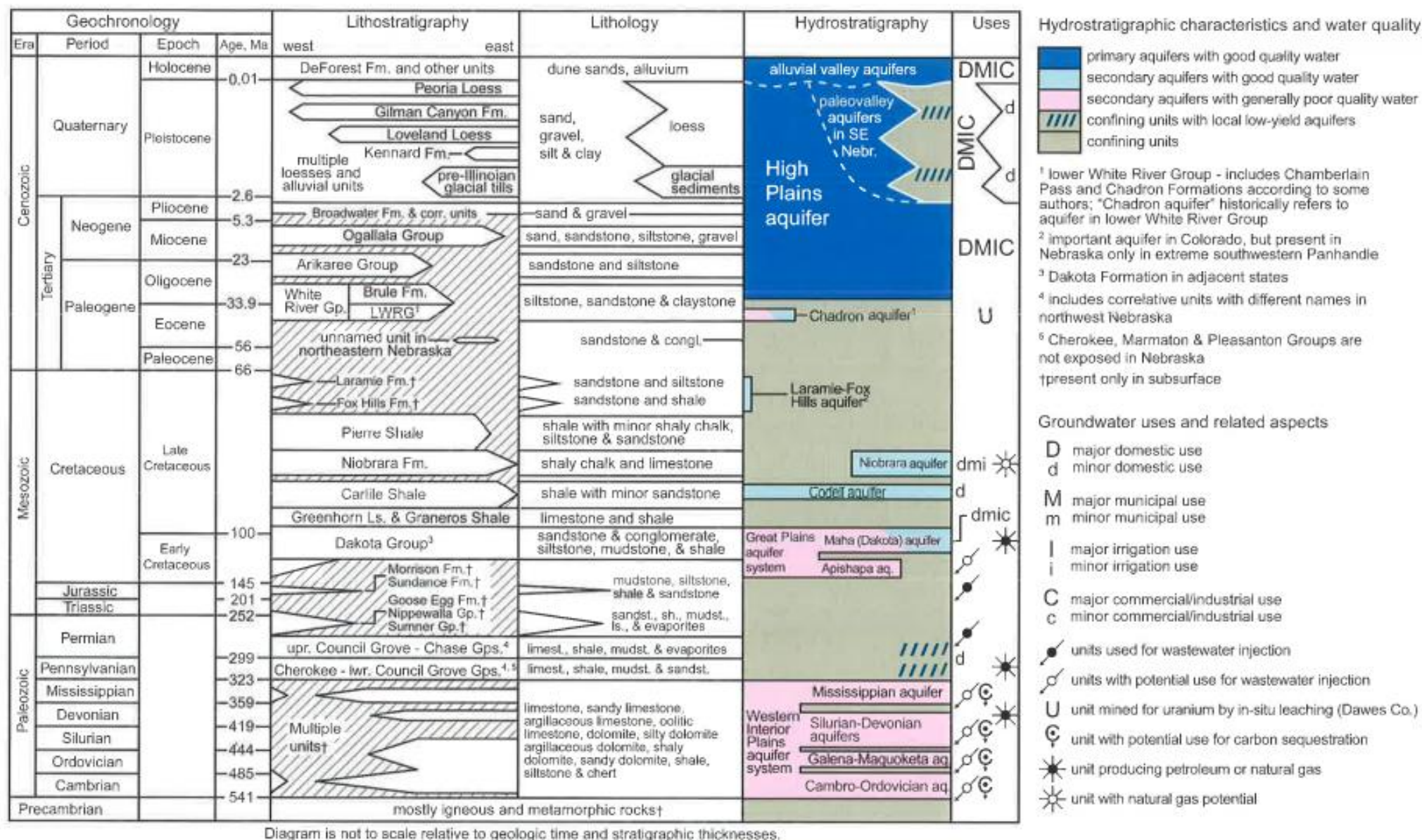
Figure 13. Generalized geologic and hydrostratigraphic framework of Nebraska.
