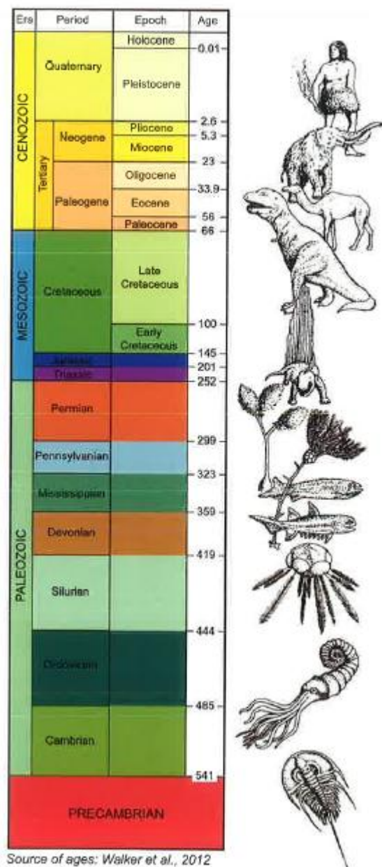
Geologic time units and age in millions of years
