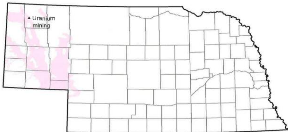
Figures 19. Areas of Nebraska underlain by the Chadron aquifer.
