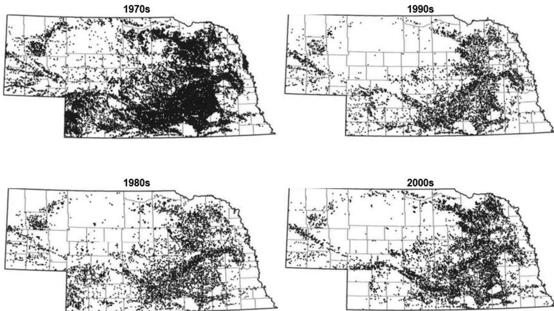
Figure 2 (continued). Locations of registered irrigation wells installed during each of the last eight full decades. Each map shows only those wells that were installed during that decade and not those wells that existed prior to that decade.
