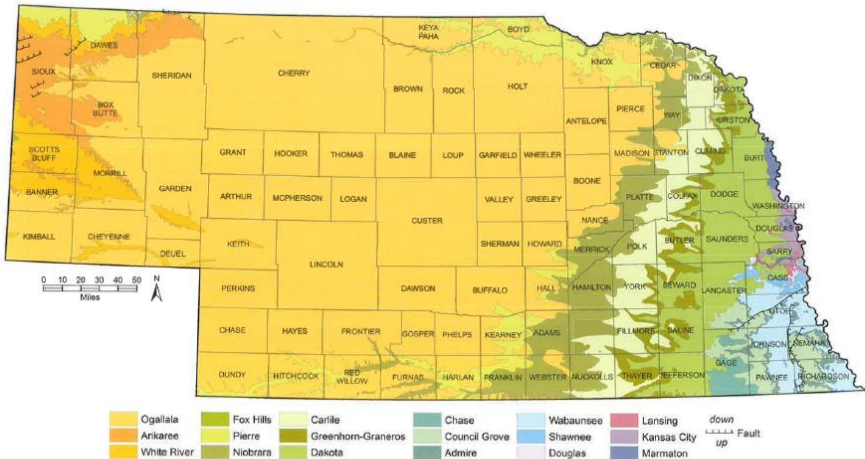
Figure 15. Geologic bedrock map of Nebraska (modified after Burchett, 1986). Pennsylvanian System includes Marmaton, Kansas City, Lansing, Douglas, Shawnee, Wabaunsee, Admire, and lower Council Grove Groups. Permian System includes upper Council Grove and Chase Groups. Cretaceous System includes Dakota Group, Greenhorn Limestone, Graneros Shale, Carlile Shale, Niobrara Formation, Pierre Shale, and Fox Hills Formation. Tertiary System includes White River, Arikaree, and Ogallala Groups.
