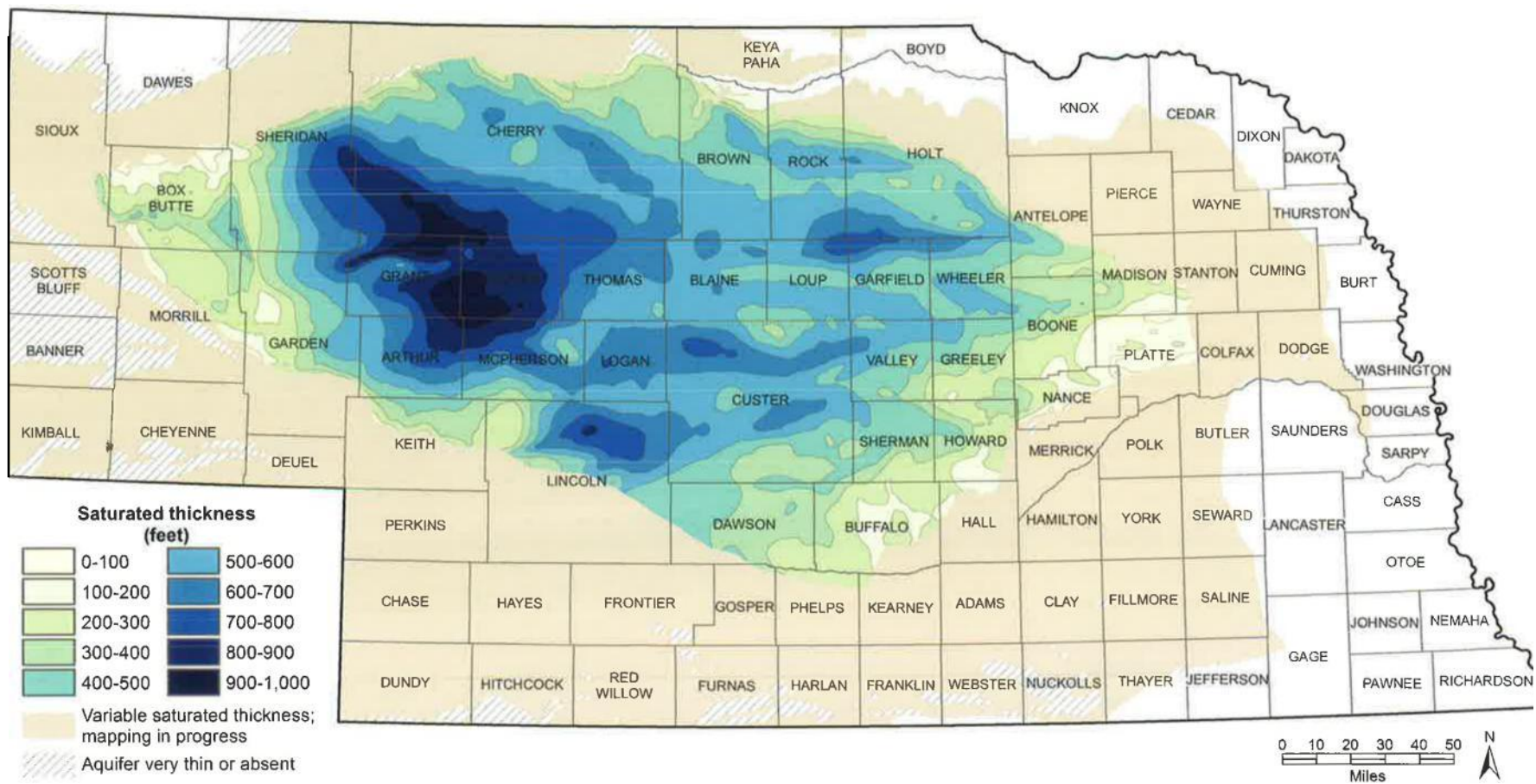
Figure 33. Saturated thickness of the unconfined portions of the High Plains aquifer. In other areas of the High Plains aquifer, the saturated thickness is highly variable and has not been mapped in detail.
