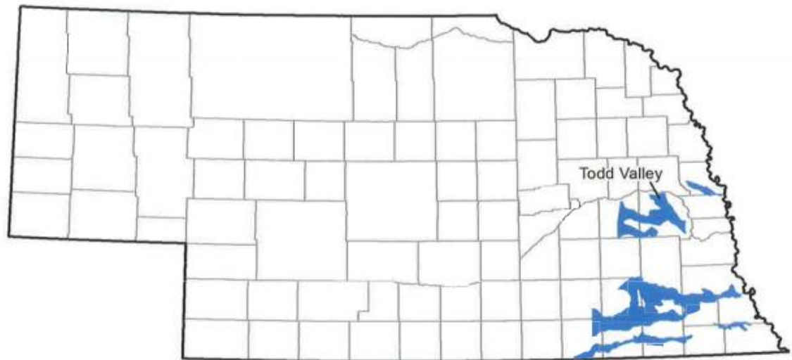
Figure 21. Areas of Nebraska underlain by paleovalley aquifers.
