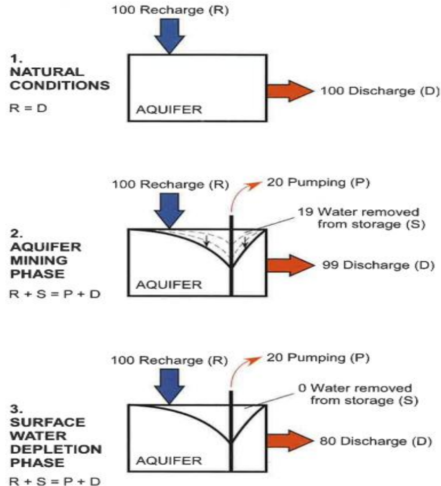
Figure 11. Conceptualization of hydrologic balance as it pertains to groundwater pumping. Numbers show arbitrary values of recharge (blue) and discharge (red). During each phase, discharge plus pumping always equals recharge plus water removed from storage. 1) Natural conditions prior to any pumping. 2) Aquifer mining phase begins immediately upon pumping and lasts until reductions in discharge become significant. 3) Surface water depletion phase begins when new water removed from storage approaches zero and lasts until pumping stops.
