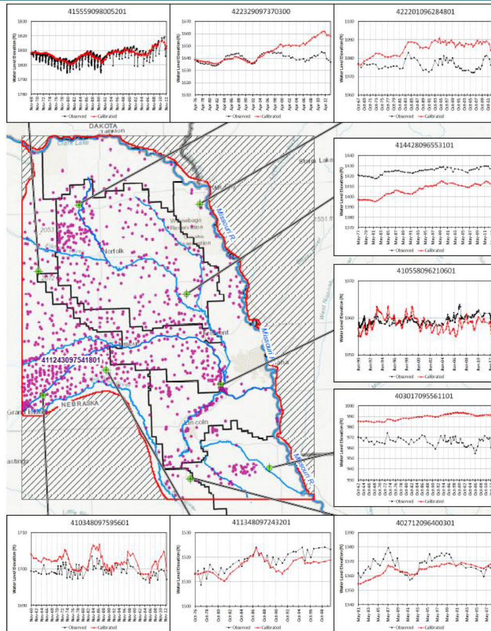
FIGURE 6-5 - COMPARISON OF SELECT SIMULATED AND OBSERVED GROUNDWATER LEVEL HYDROGRAPHS
